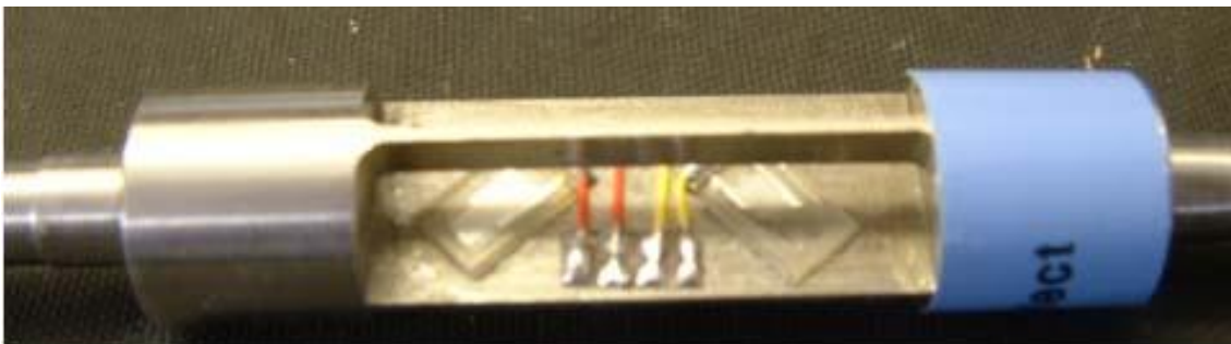
Figure 6 A typical structure - Shaft with two SAWs attached
