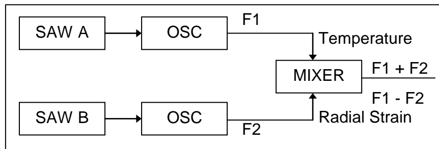
Figure 4 Schematic Of Frequency Domain SAW Signals
