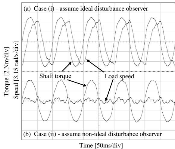
Figure 13. Experimental regulation responses with disturbance feedback; \omega_{ob} = 1.5\omega_j
