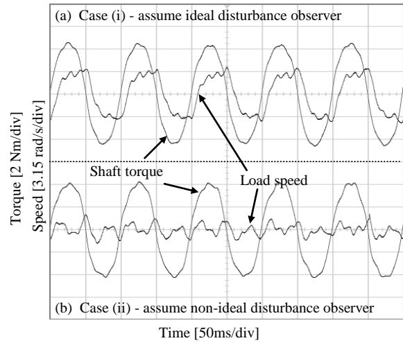
Figure 12. Experimental regulation responses with disturbance feedback; \omega_{ob} = 3\omega_j
