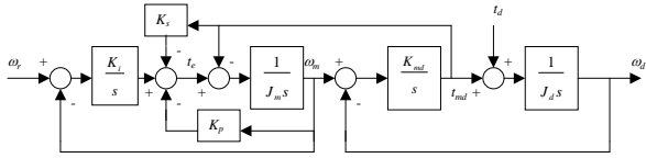
(b) RRC controller
