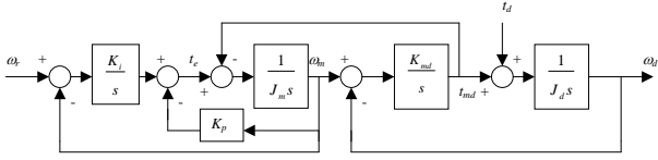
(a) PI-type controller
