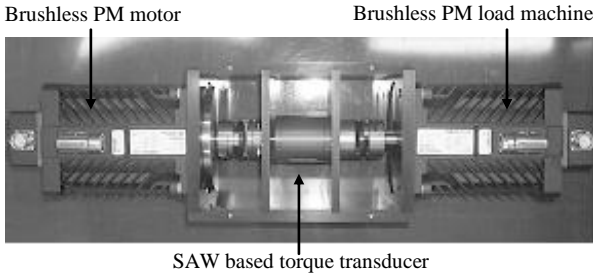
(a) Mechanical system overview
