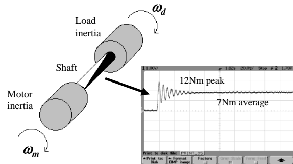
Figure 1. Measured shaft torsional oscillation immediately after the application of a 7Nm step load change.
