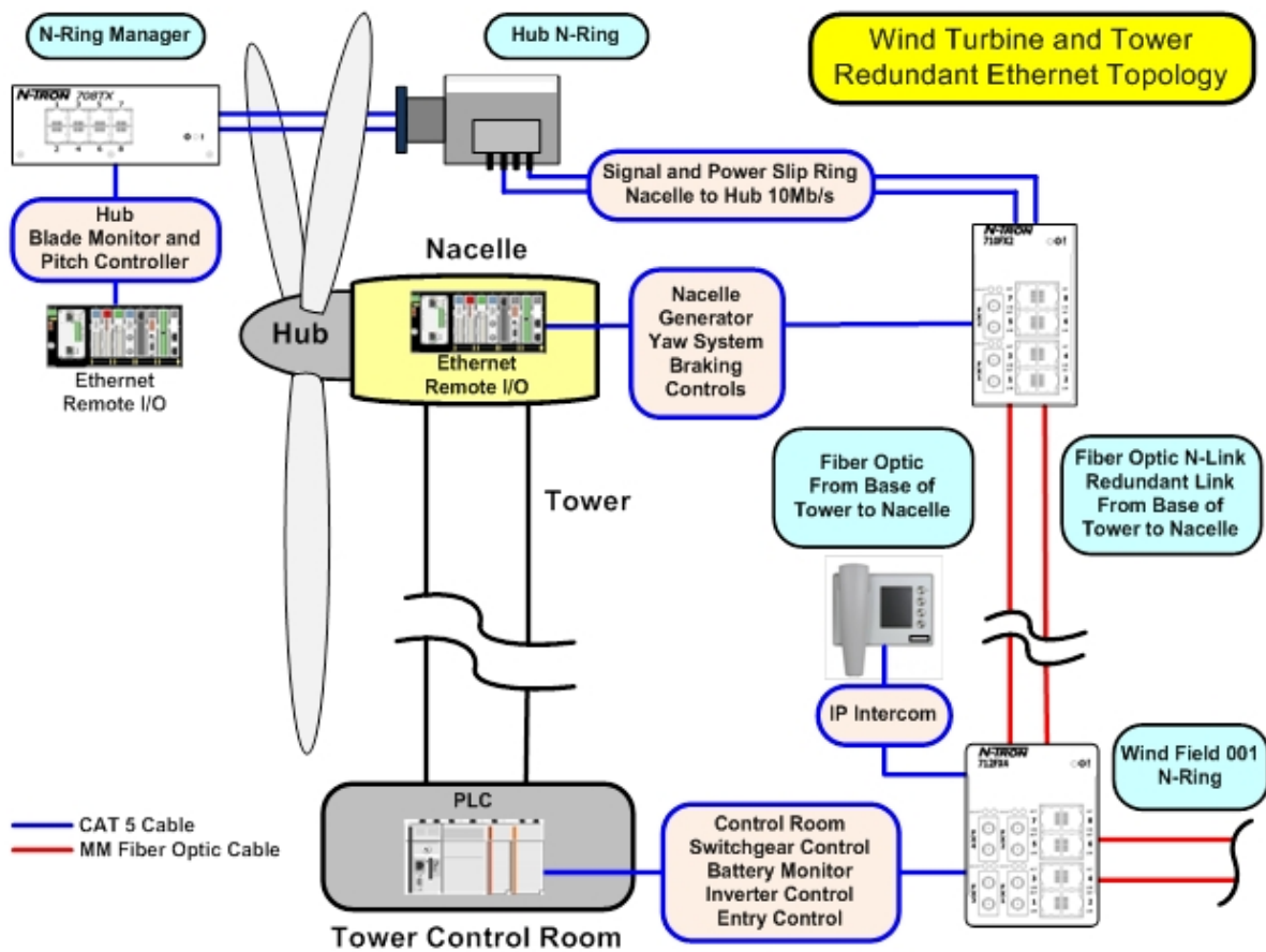
Figure 1. Wind Turbine & Tower Redundant Ethernet Topology
