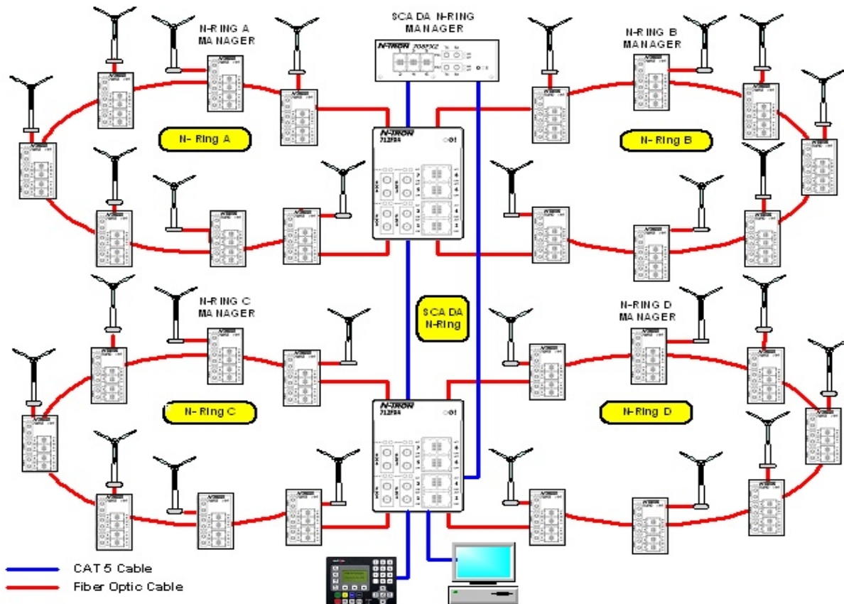
Figure 2. Wind Turbine Network Devices
