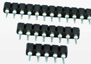
P/N:2150-XXE(2.54mm) Dwg:2150-001
