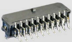
P/N:4312-SXX2RC-RN Dwg:4312-2RM
