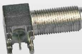
P/N:3296 Dwg:3296-001
