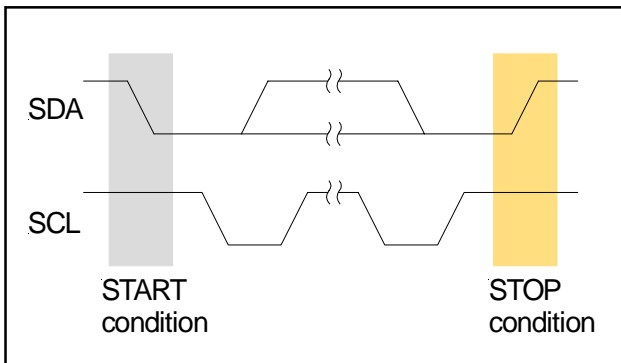
Fig. 4: I 2 C bus START and STOP conditions
