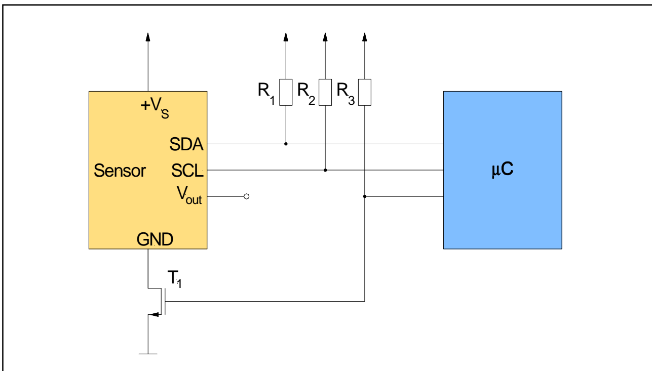
Fig. 13: Circuit for I 2 C reset
