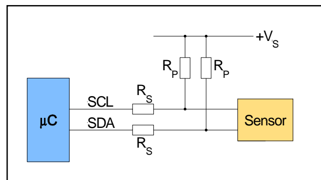
Fig. 12: I 2 C bus application circuit for HMI, HDI, HCLA, HCA and SSI pressure sensors
