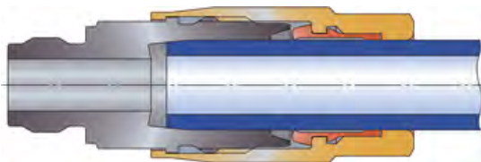
Tube, disconnected
